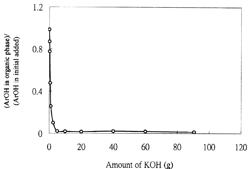
Figure 4 Relation between the concentration of ArOH in the organic-phase and the amount of KOH; 8 g of 2,4,6-tribromophenol (ArOH), 1 g of QBr (TBAB) catalyst, 25 mL of water, 100 mL of dichloromethane, 293 K, 700 rpm
