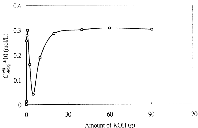
Figure 2 The dependence of the concentration of ArOQ on the amount of KOH in the two-phase reaction (same reaction conditions as given in Figure 1)
