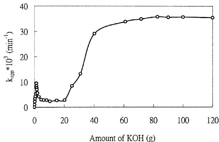
Figure 1 Relation between apparent rate constant ( k_{app} ) and the amount of KOH in the two-phase reaction; 8 g of 2,4,6-tribromophenol (ArOH), 0.01 mol of \alpha -bromo- o -xylene (RBr), 1 g of TBAB (QBr) catalyst, 25 mL of water, 100 mL of dichloromethane, 293 K, 700 rpm
